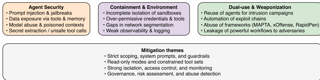
FIGURE 12. Conceptual taxonomy (illustrative, derived from the surveyed safety and governance literature) of three risk dimensions for LLM-based security agents: agent security, containment, and dual-use; together with common mitigation themes such as scoping, isolation, and governance.
