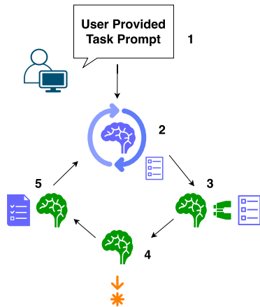
FIGURE 1. Conceptual Plan-then-Execute architectural diagram (illustrative, synthesized from surveyed literature) showing the interaction between Planner and Executor agents.
