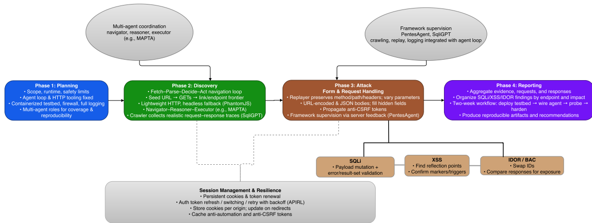
FIGURE 2. Conceptual four-phase workflow (illustrative, synthesized from surveyed frameworks) for LLM-based web and API penetration testing: planning, discovery, attack, and reporting.
