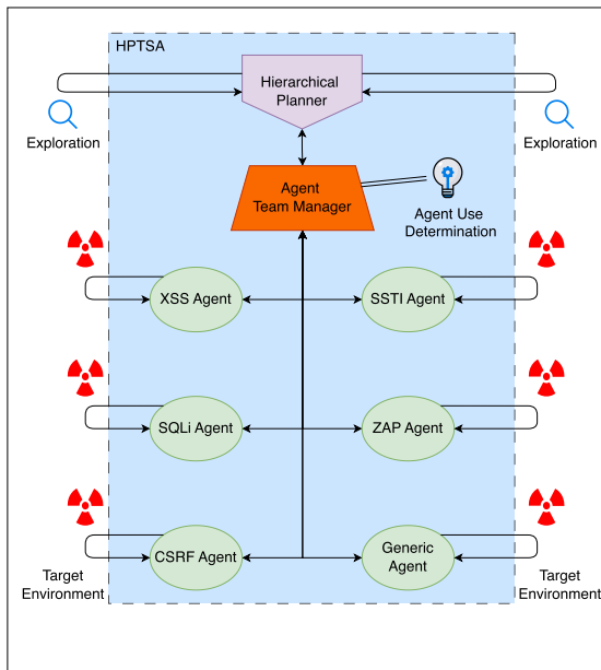
FIGURE 4. Conceptual HPTSA interaction architecture (illustrative, synthesized from the source description) showing hierarchical planning agent, management agent, and task-specific expert agents.
