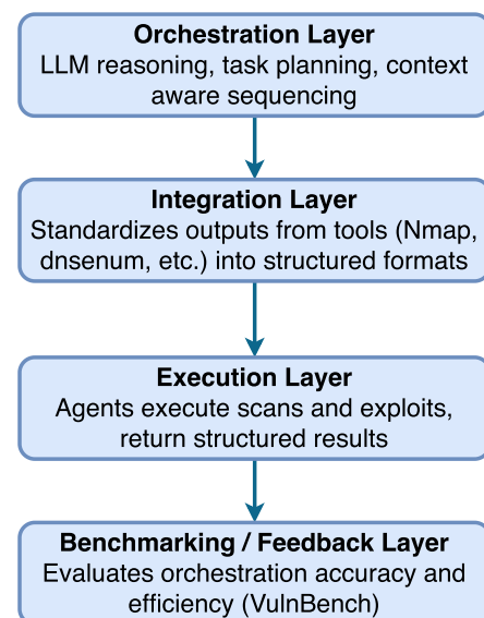
FIGURE 7. Conceptual layered architecture (illustrative reference model, synthesized from surveyed frameworks) of an AI agentic penetration testing system.
