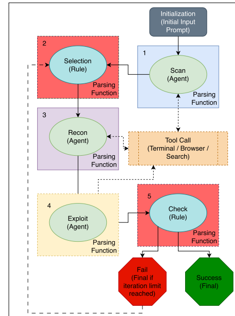
FIGURE 3. Conceptual AutoPT FSM workflow (illustrative, synthesized from source descriptions) showing state transitions between scanning, reconnaissance, and exploitation phases.
