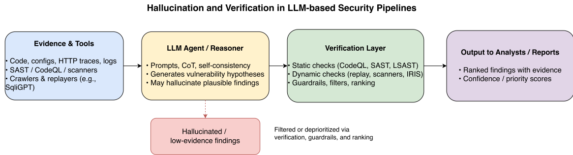
FIGURE 10. Conceptual verification pipeline (illustrative, synthesized from surveyed approaches) for LLM-generated vulnerability hypotheses: static and dynamic analysis layers filter hallucinated or false-positive findings before analyst review.
