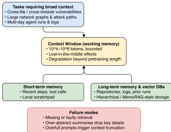
FIGURE 11. Conceptual memory architecture (illustrative reference model) for LLM-based security agents: short-term working context (bounded by token limits) augmented by long-term retrieval systems that selectively surface relevant information.
