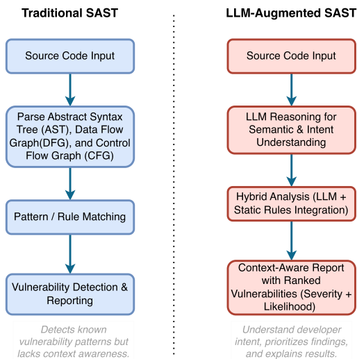
FIGURE 6. Conceptual evolution of Static Application Security Testing architectures (illustrative comparison) from traditional SAST to LSAST with RAG.
