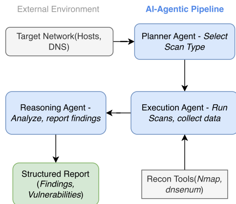
FIGURE 8. Conceptual orchestration diagram (illustrative, synthesized from surveyed frameworks) of agentic network scanning, showing interaction between an LLM-based agent, reconnaissance tools (Nmap, dnsenum), and the target network environment.
