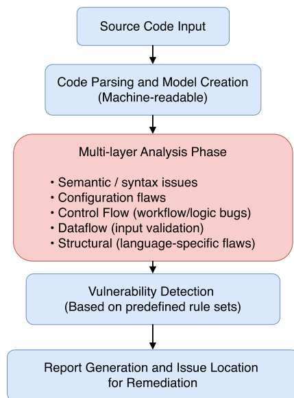
FIGURE 5. Conceptual workflow of Static Application Security Testing (illustrative summary of typical SAST stages, not a benchmark of any specific tool).
